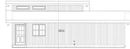
Front Elevation
