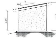
Left Elevation
