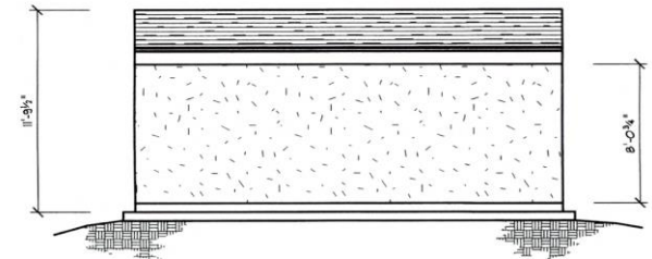
Back Elevation
