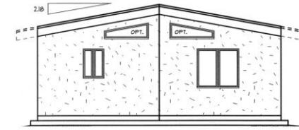
Rear Elevation
