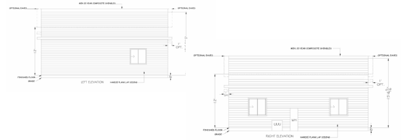
Side Elevations
