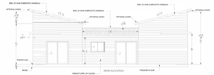
Back Elevation
