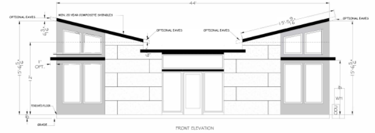
Front Elevation
